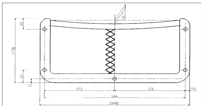
620 0097 Plastic Frame Net
