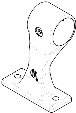
("DL" VERSIONS ONLY) ISOMETRIC VIEW SCALE: 1:2
