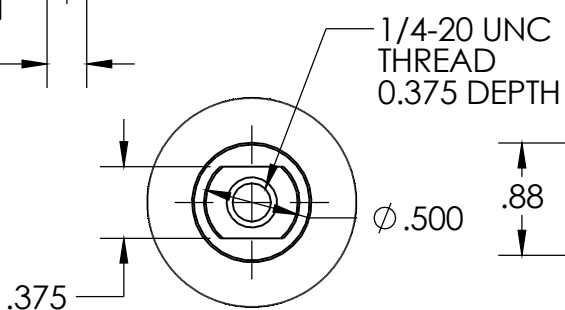
VIEW A-A SCALE 1 : 1
