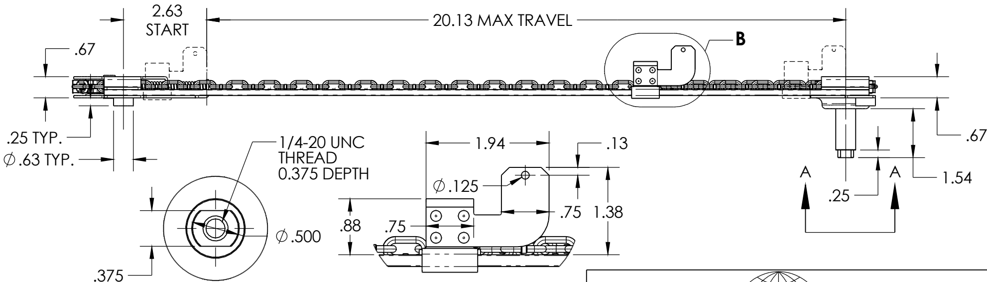
VIEW A-A SCALE 1 : 1
