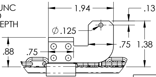
DETAIL B SCALE 2 : 3
